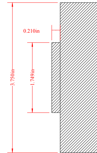
Crank Side View
