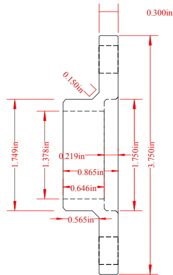
Spacer Side View
