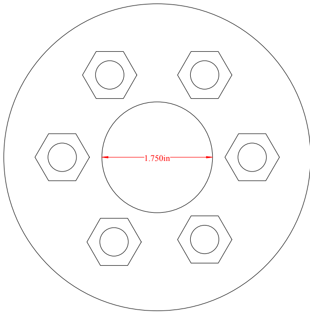
Flywheel
