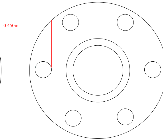
Spacer Rear View
